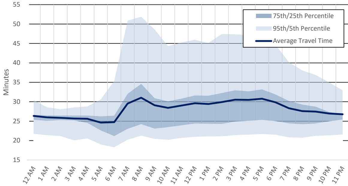
Figure 8: Average Northbound Travel Times between Rockville and Clarksburg (2018)
