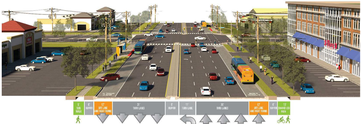
An example of a curb lane transitway
