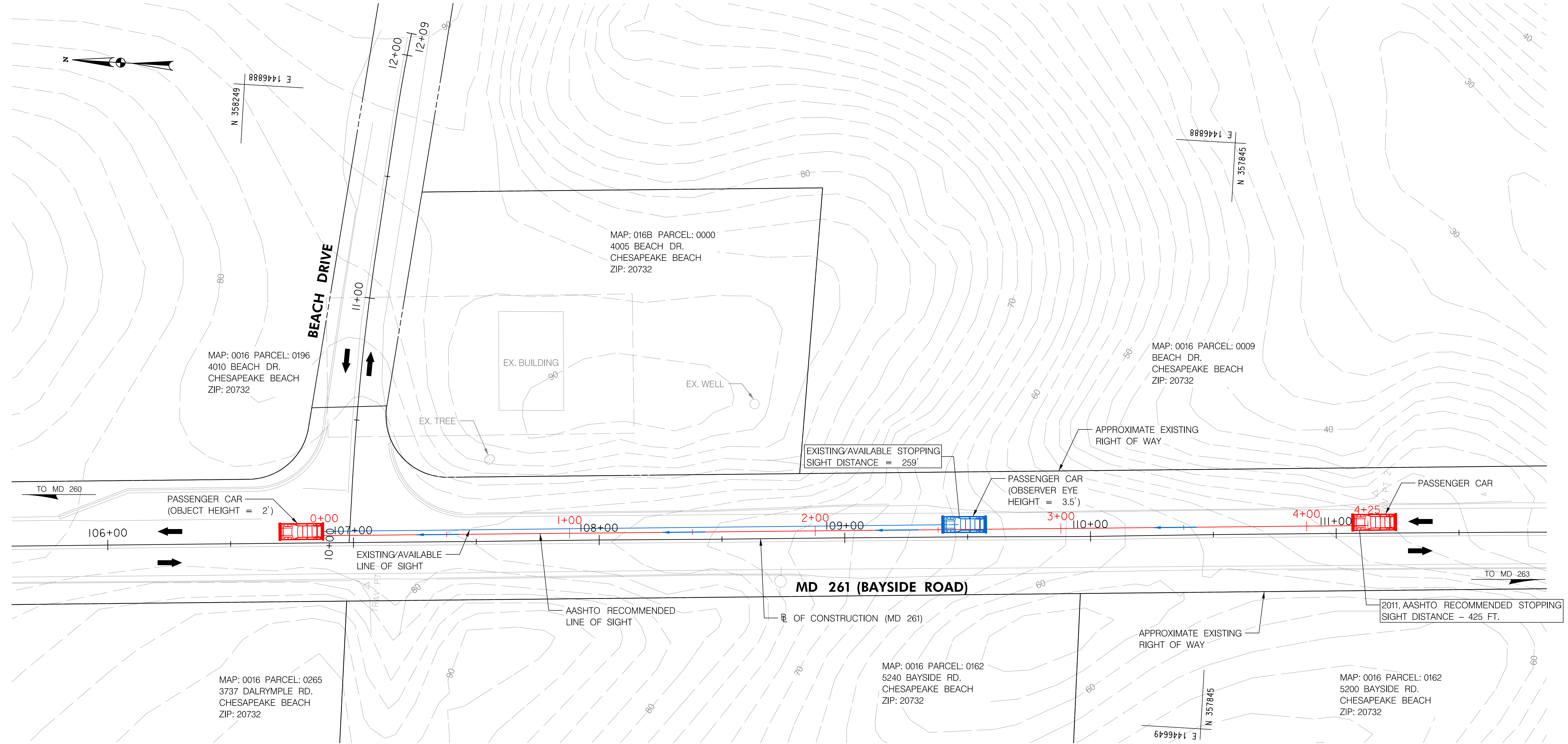
STOPPING SIGHT DISTANCE (MD 261 – NORTHBOUND)
