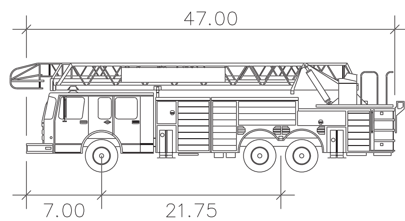
Fire Truck MC AT-29
