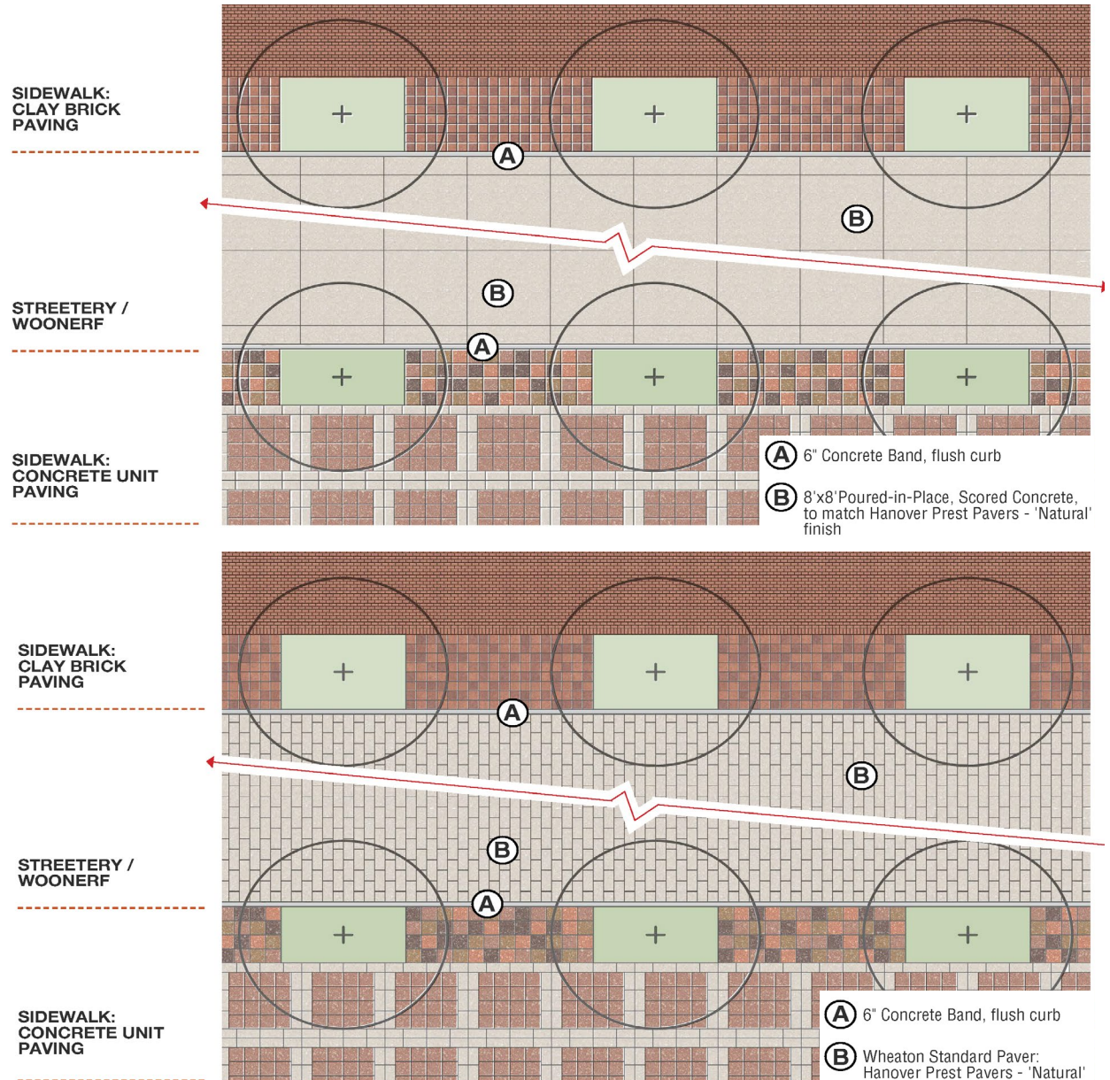
Figure 17: Alternatives for full shared street pavement
