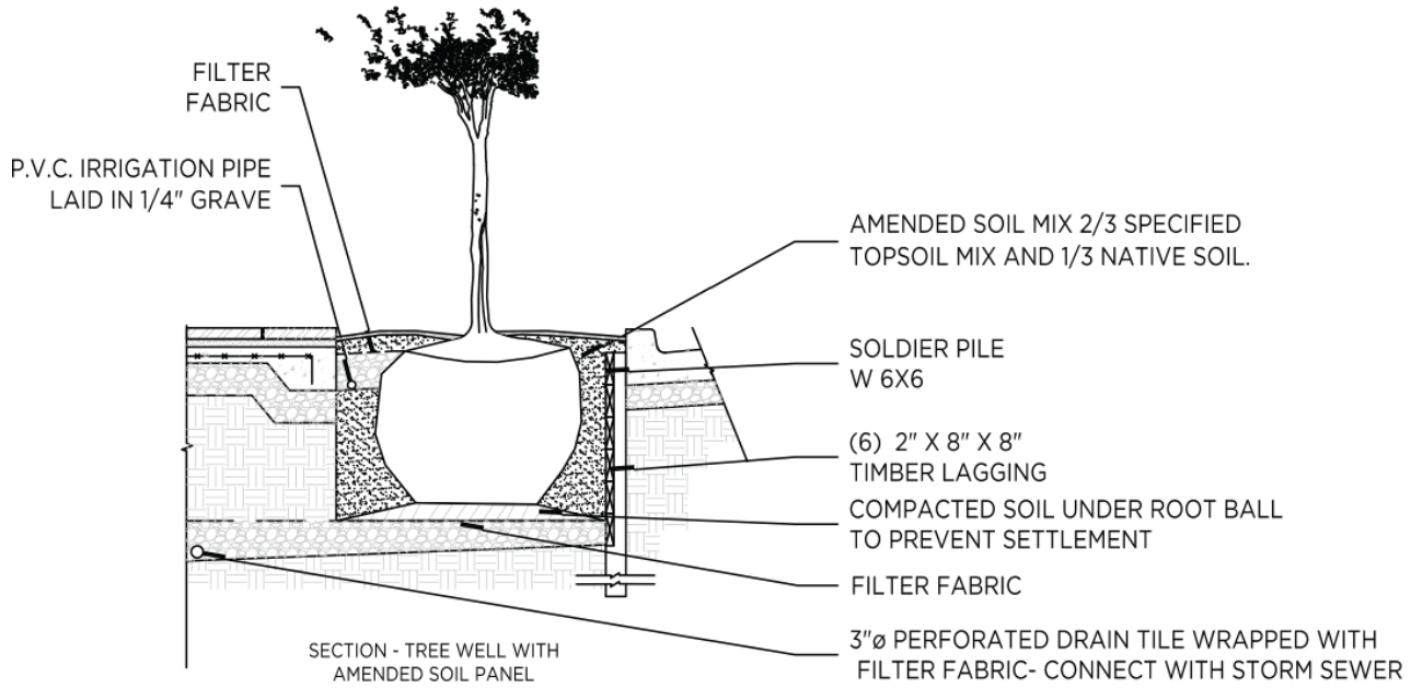
General Tree Planting Detail
