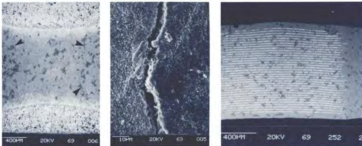
(a) Macrophotograph: arrows show surface cracks (b) Closeup of a 0.002-inch crack (c) Cross section of (a) indicates that the cracks extend through the surface defect to the first metal electrode
