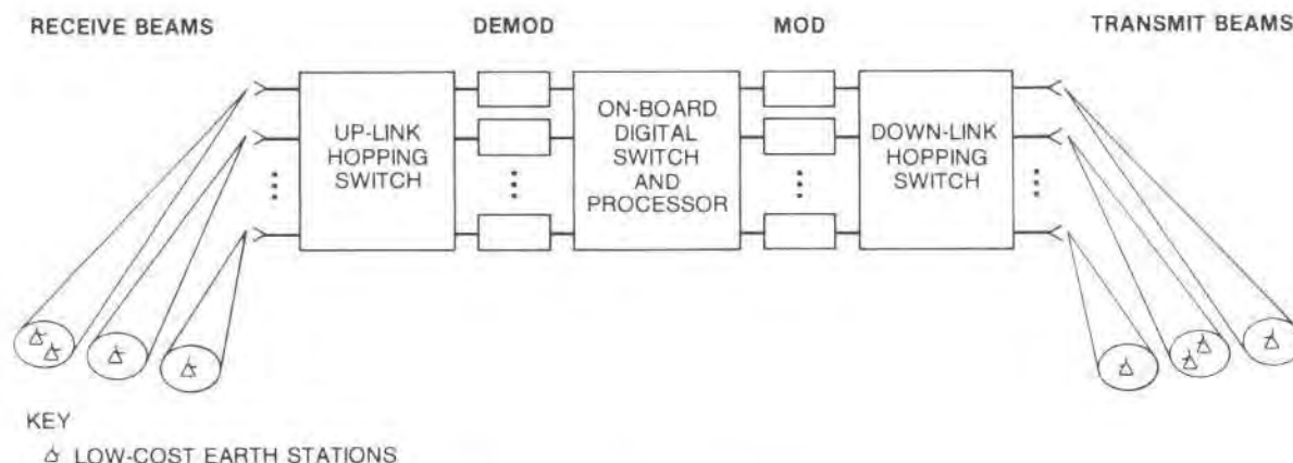
Figure 6. Multibeam satellite with baseband processing reduces earth station costs
