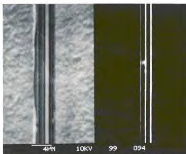
Figure 12. COMSAT-fabricated GaAs power FET operated near breakdown point (a) Secondary electron image (b) Electron-beam-induced current image
