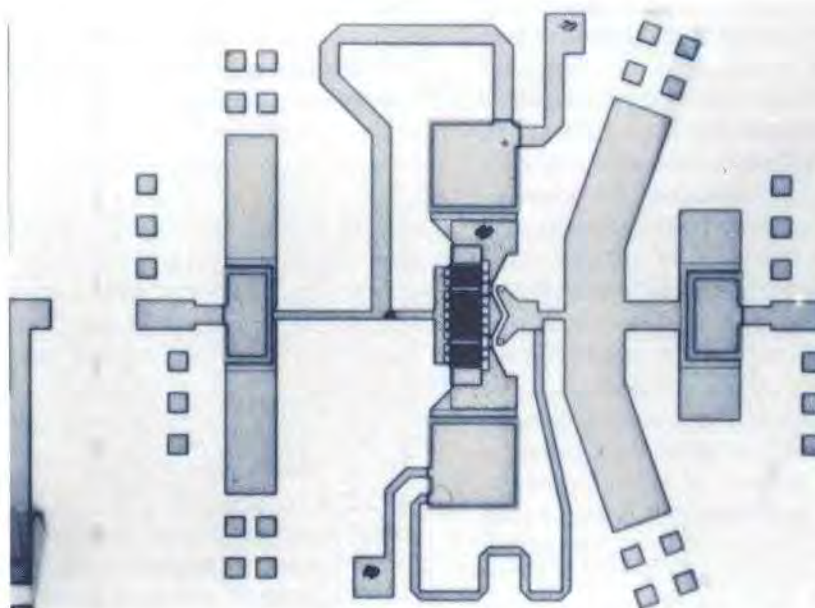
Figure 9. Single- and dual-stage 20-GHz MMIC amplifiers deliver 0.5 W at 4- and 8-dB gain, respectively
