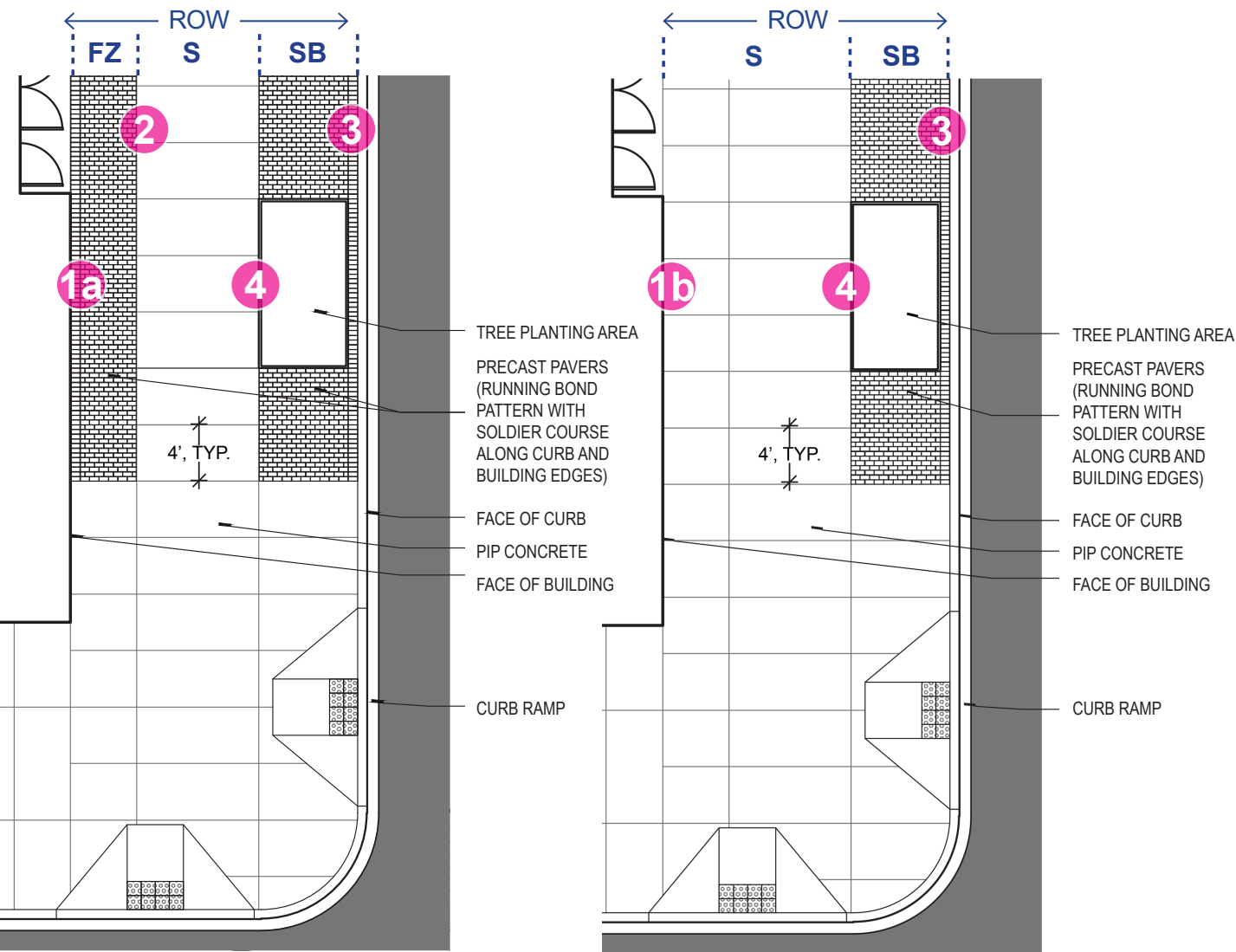
Figure 4: Typical streetscape paving plans for streets with and without Frontage Zones (FZ)
