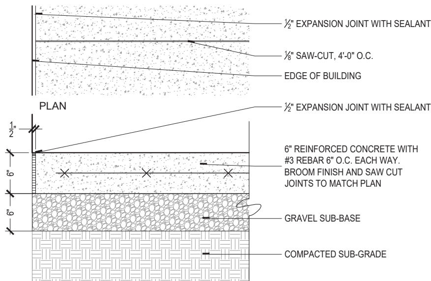
1b Detail 1b: Poured-in-place concrete sidewalk at building face (no Frontage Zone)
