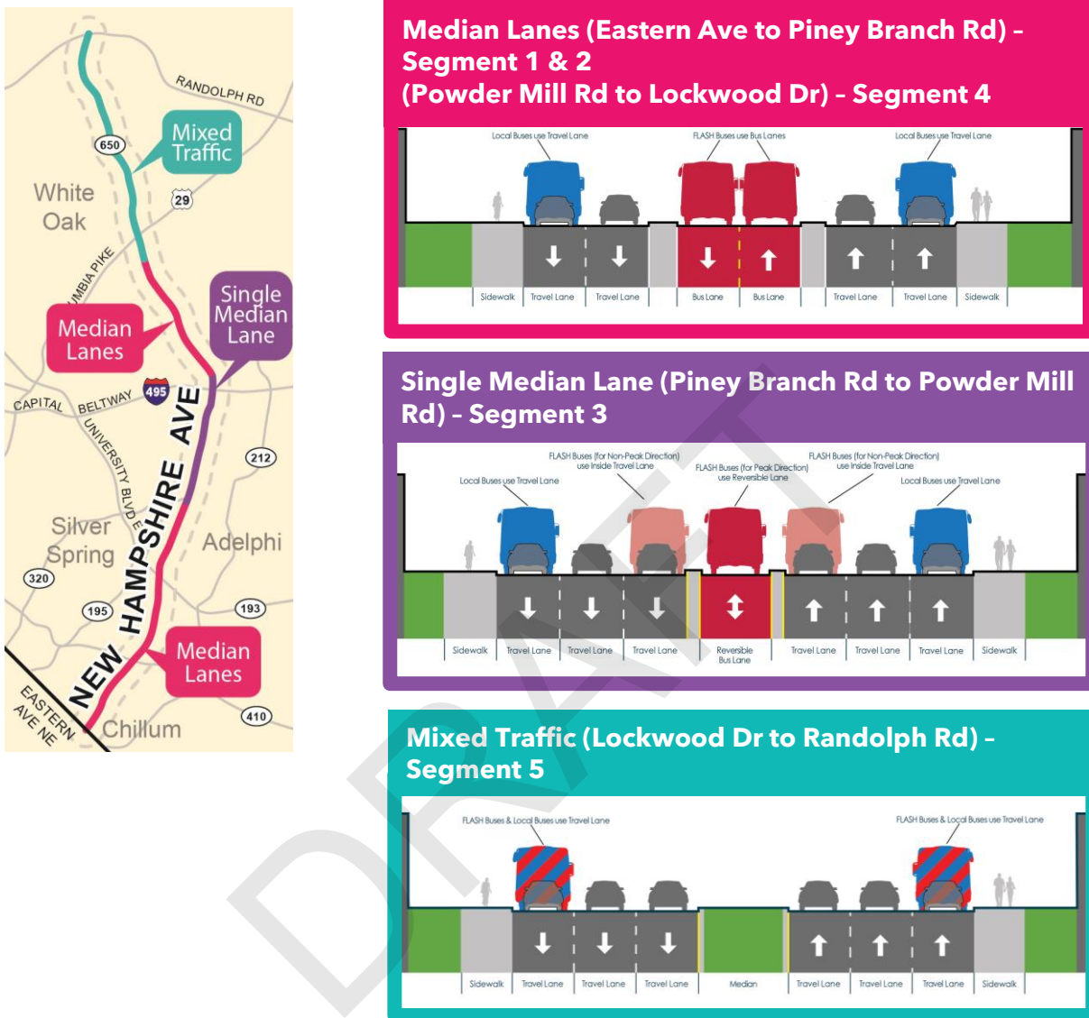
Figure 42: Alternative 4 - Additional Median Lanes
