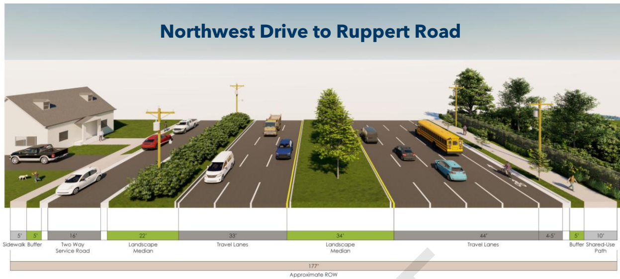
Figure 26: Segment 4 Existing Typical Section (northern end)
