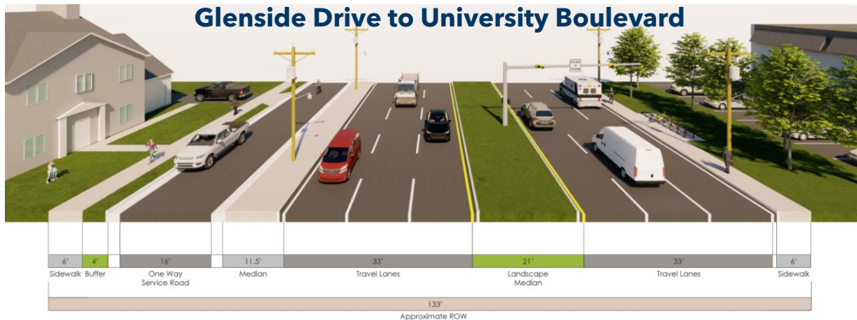
Figure 22: Segment 1 Existing Typical Section (northern end)
