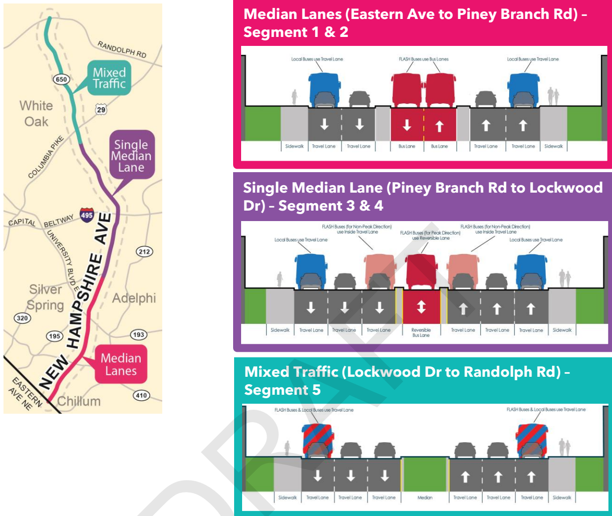
Figure 41: Alternative 3 – Median Lanes
